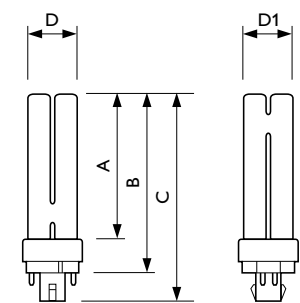
PL-C 26W/830/4P
