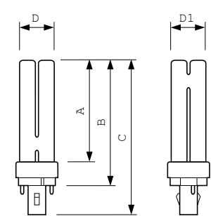
PL-C 26W/840/2P
