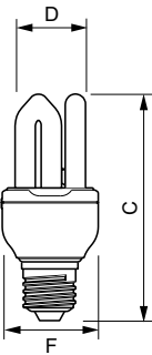
Econ Genie ErP NG 11W/827 E27 220-240V
